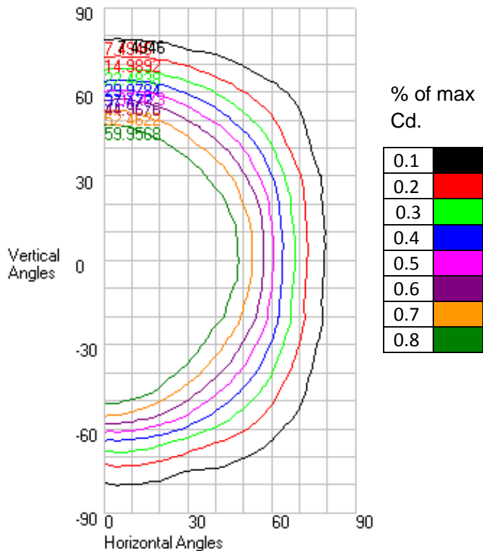
Isocandela
